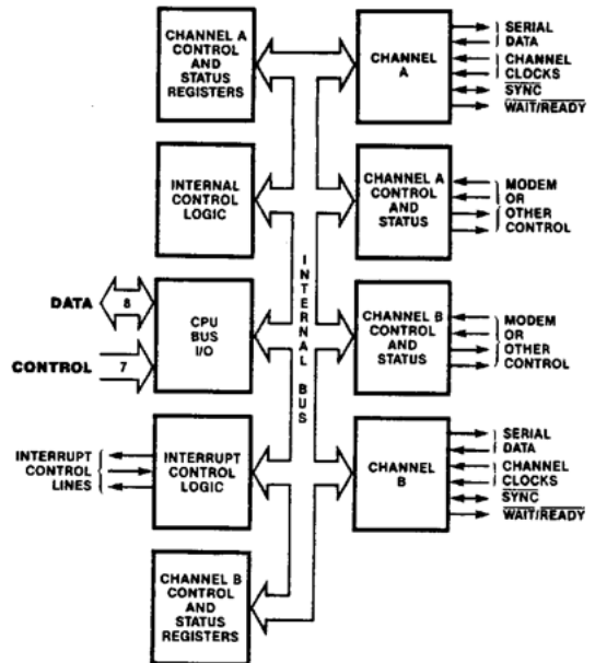
Figure 8. Block Diagram
