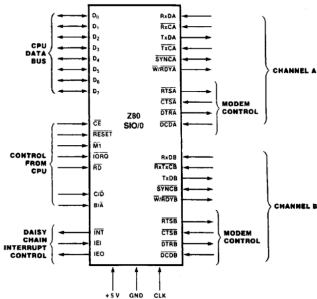
Figure 5. Pin Functions
